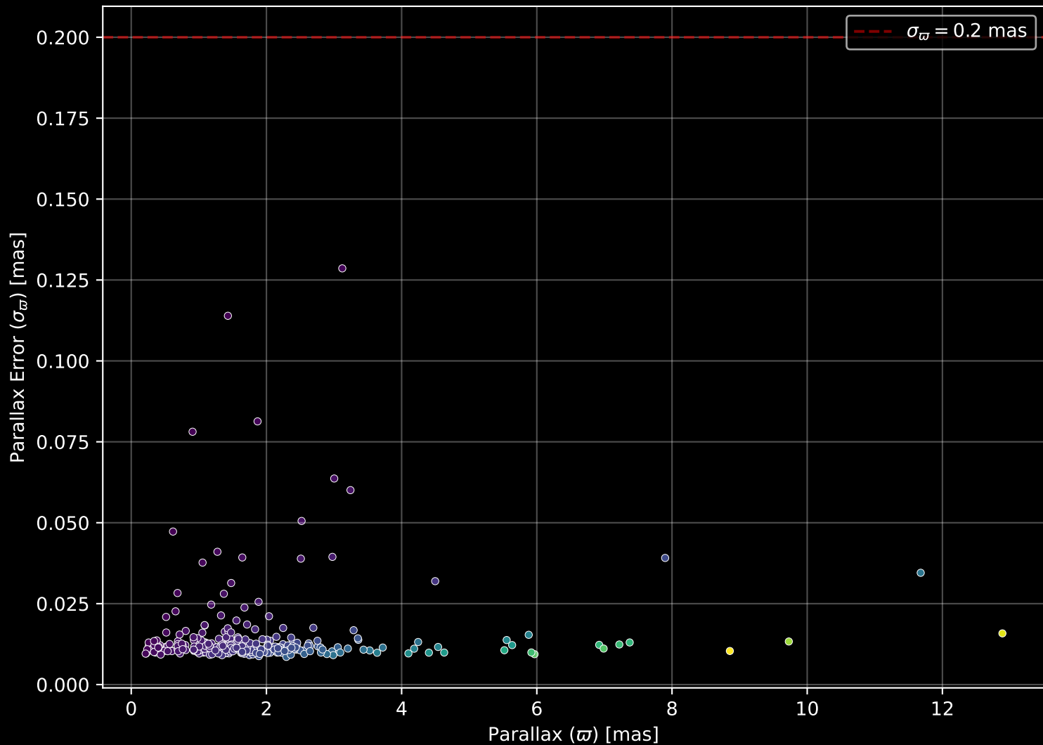
GALAH DR4 Field: [302] Parallax Quality (n= 293)
