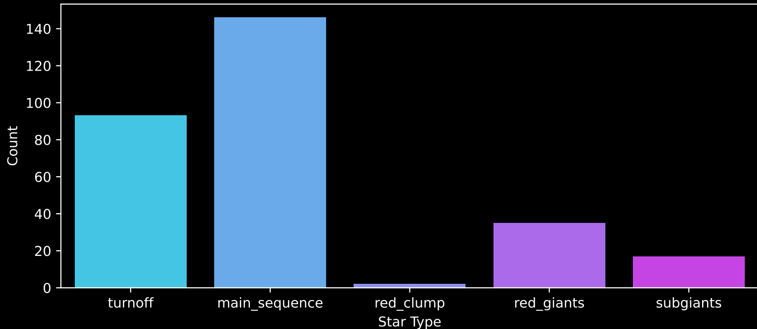
GALAH DR4 Field: [302] Count plot of Star Type
