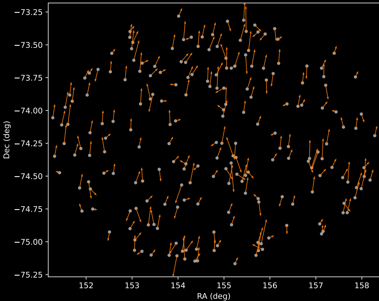
GALAH DR4 Cluster 2 Proper Motion Vectors (n=207)
