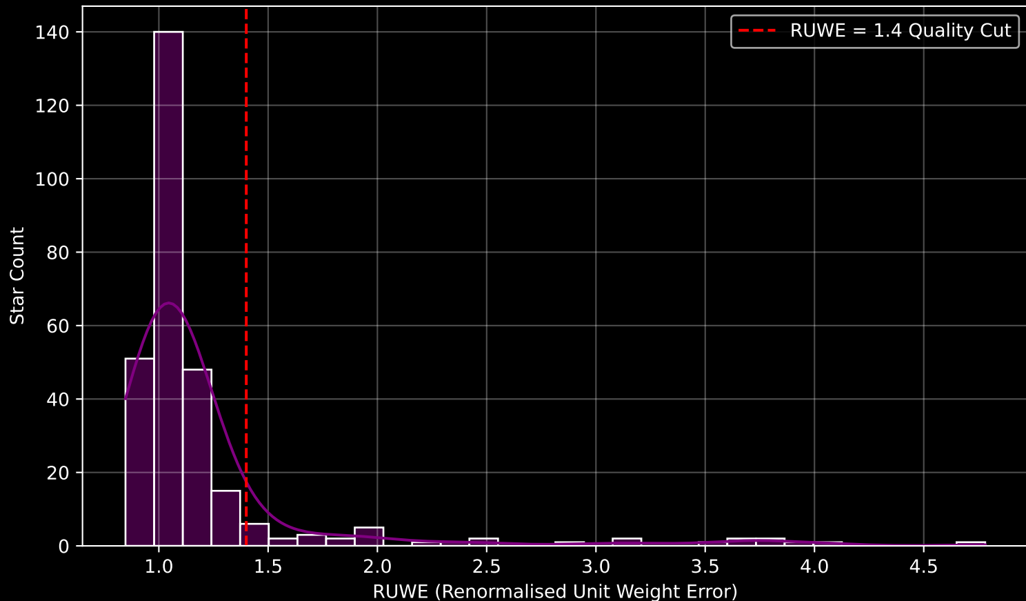
GALAH DR4 Field [302] RUWE Distribution (n= 287)
