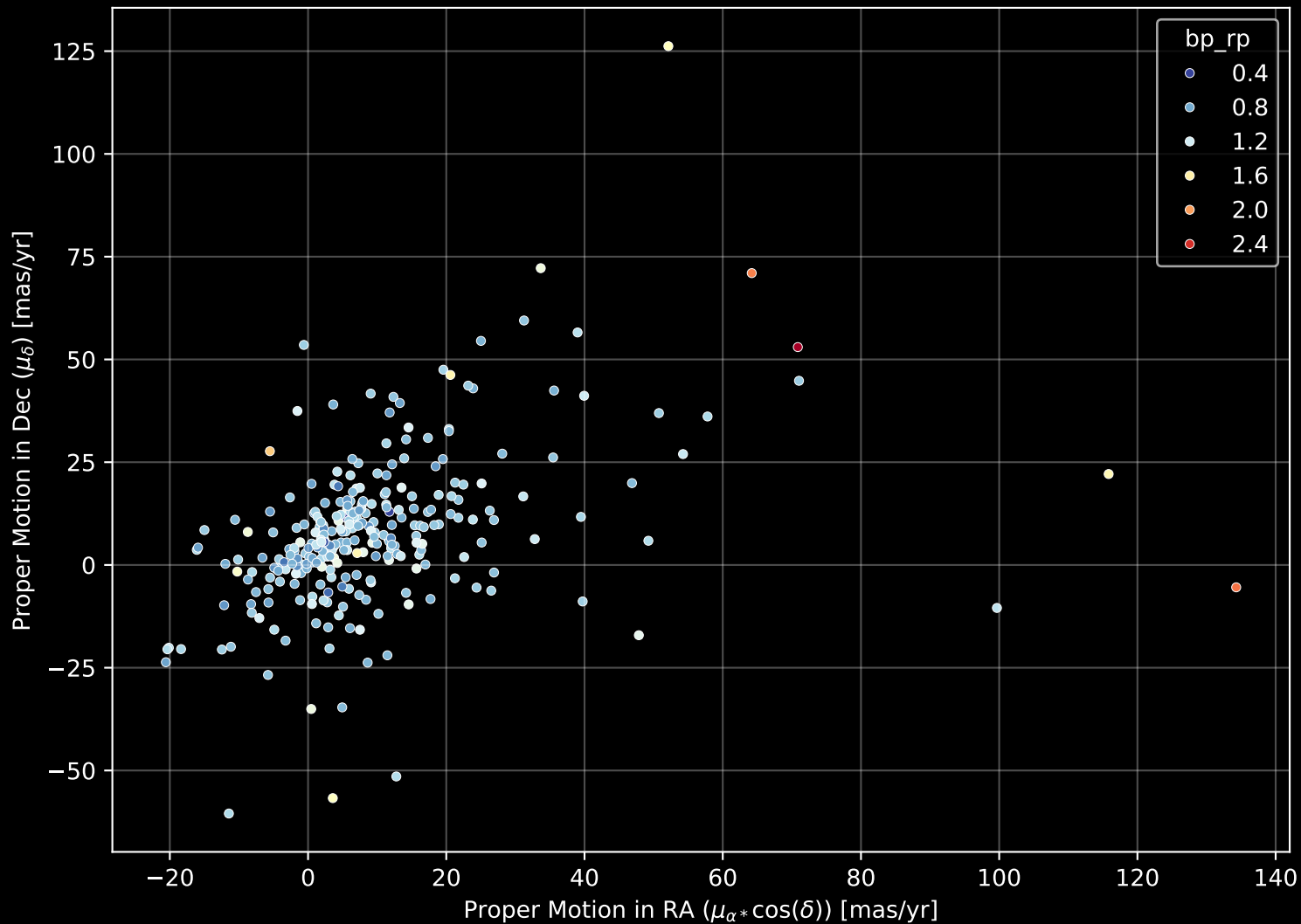
GALAH DR4 Field: [302] Proper Motion Diagram (n= 293)
